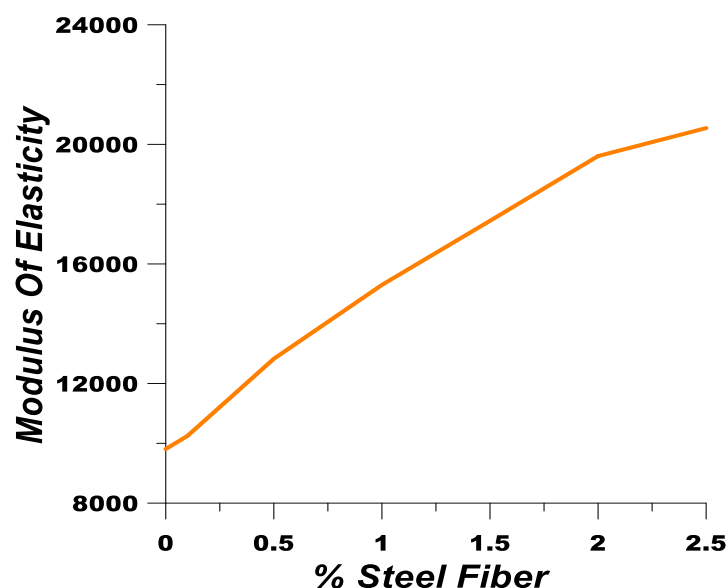
Fig. 11 Modulus Of Elasticity Test
