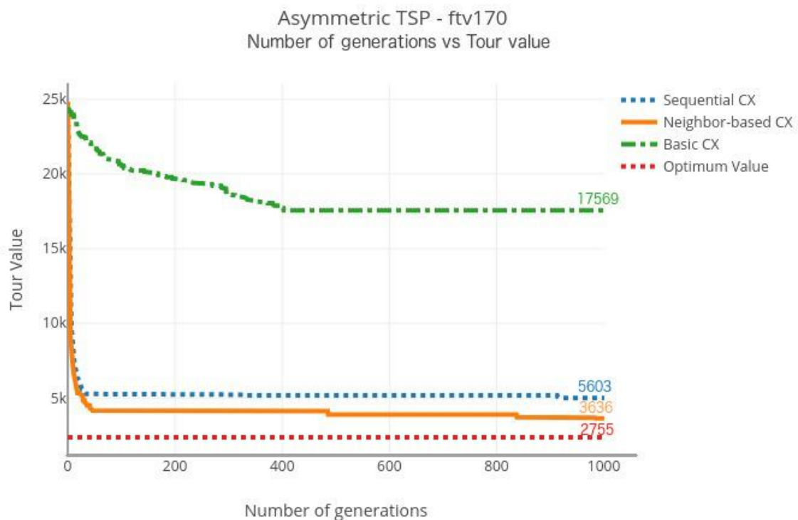
Figure 2. Performance of different crossover operators on Asymmetric TSP instance fvt70(71 nodes) [2]
