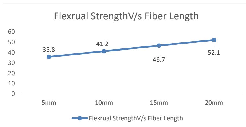
Figure 5. Graph between flexural strength and fiber length
