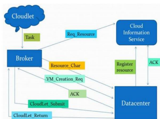
fig 2 cloud architecture
