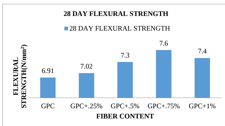
Fig 3.3 Flexural strength results
