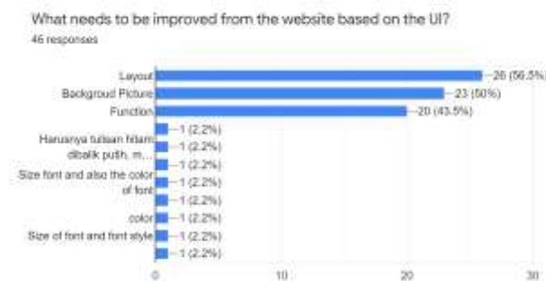
Figure 7. Users responses
